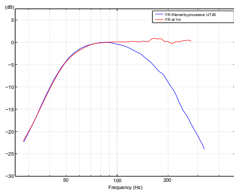
Frequency response at 1m
