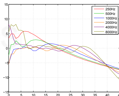
Abscissa: distance (m). Column SA250P at 2,55m from ground. 0 dB is the mean SPL over 10m-30m on axis.
