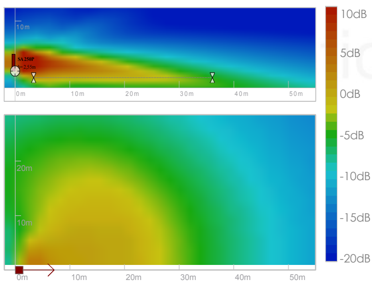
Abscissa: distance (m). Column SA250P at 2,55m from ground. 0 dB is the mean SPL over 10m-30m on axis.
