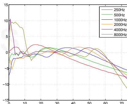
Abscissa: distance (m). Column SA400P at 2,55m from ground. 0 dB is the mean SPL over 10m-45m on axis.
