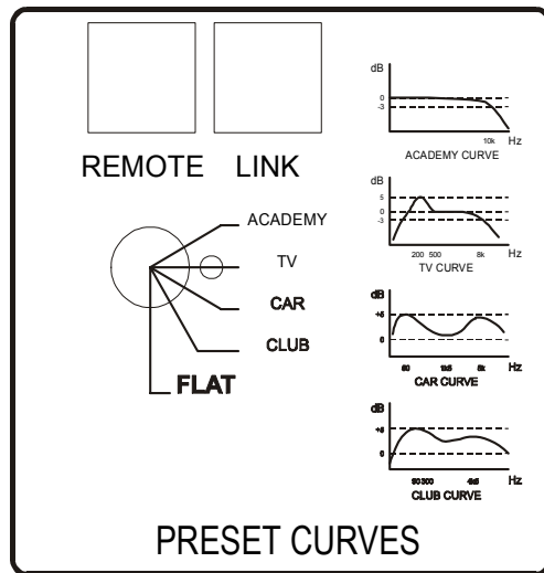
Figure 5: preset curves
