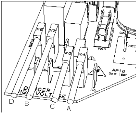
Main power 110/120 VAC
