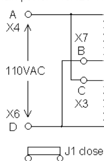
Main power 110/120 VAC
