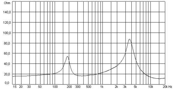
XS 5.1 Impedance curve
