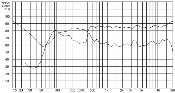
XS 5.1 Frequency Response + Phase
