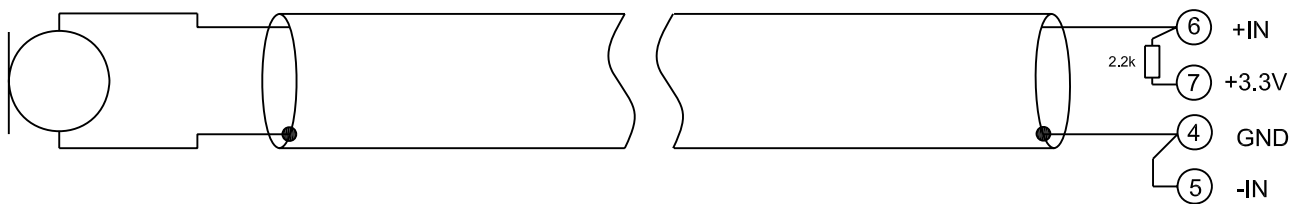
Electret 2 wires R=2.2k - DPA 4063
