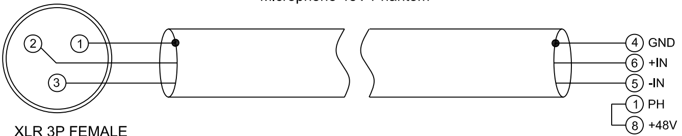
Microphone 48V Phantom
