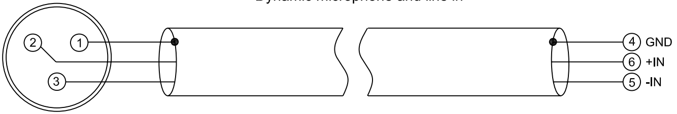
Dynamic microphone and line in
