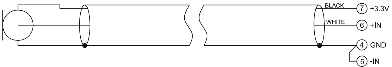
Electret 3 wires SANKEN COS11
